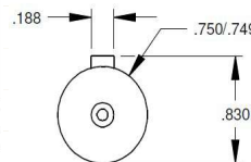
3/4" KEYED SHAFT (CODE 4)
